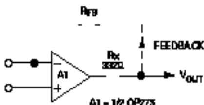
Figure 1. Recommended Output Short Circuit Protection
