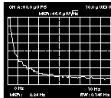
Figure 6. 1/f Noise Corner, V_S = \pm 15 V, A_V = 1000
