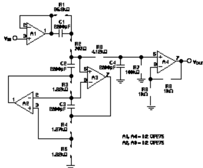
Figure 18. A 3-Pole, 40 kHz Low-Pass Filter
