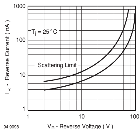
Figure 2. Reverse Current vs. Reverse Voltage
